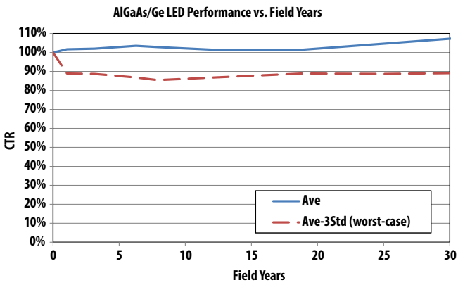
Figure 5: CTR Performance vs. Field Years for AlGaAs/Ge LED (Operating I_F = 12 mA, 50% Duty Cycle, T_A = 80^\circ\text{C} )
