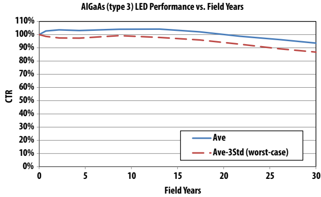
Figure 3: CTR Performance vs. Field Years for AlGaAs (Type 3) LED (Operating I_F = 12 mA, 50% Duty Cycle, T_A = 110^\circ\text{C} )
