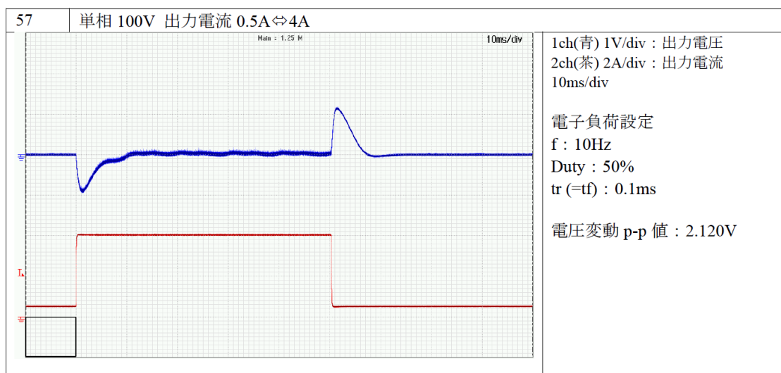
図 8-5 負荷応答性 [单相 100V, I out :0.5A⇄4A]
